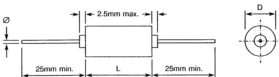
FIGURE 2 - PHYSICAL DIMENSIONS
