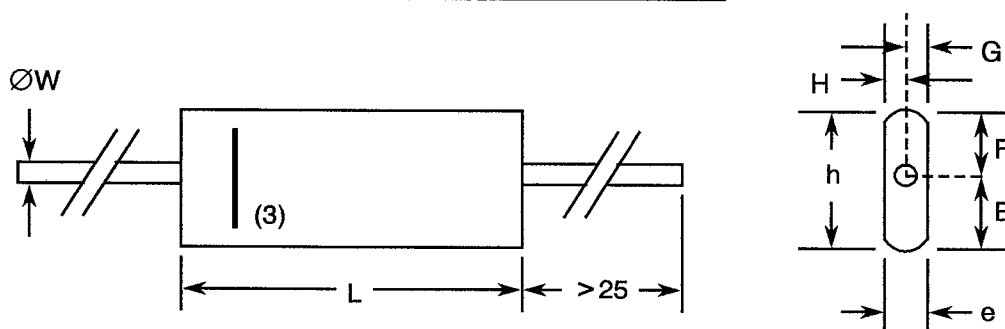
FIGURE 2 - PHYSICAL DIMENSIONS
