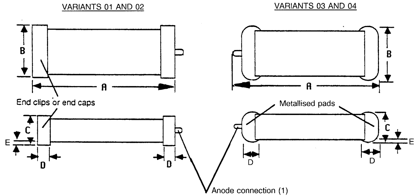
FIGURE 2 - PHYSICAL DIMENSIONS
