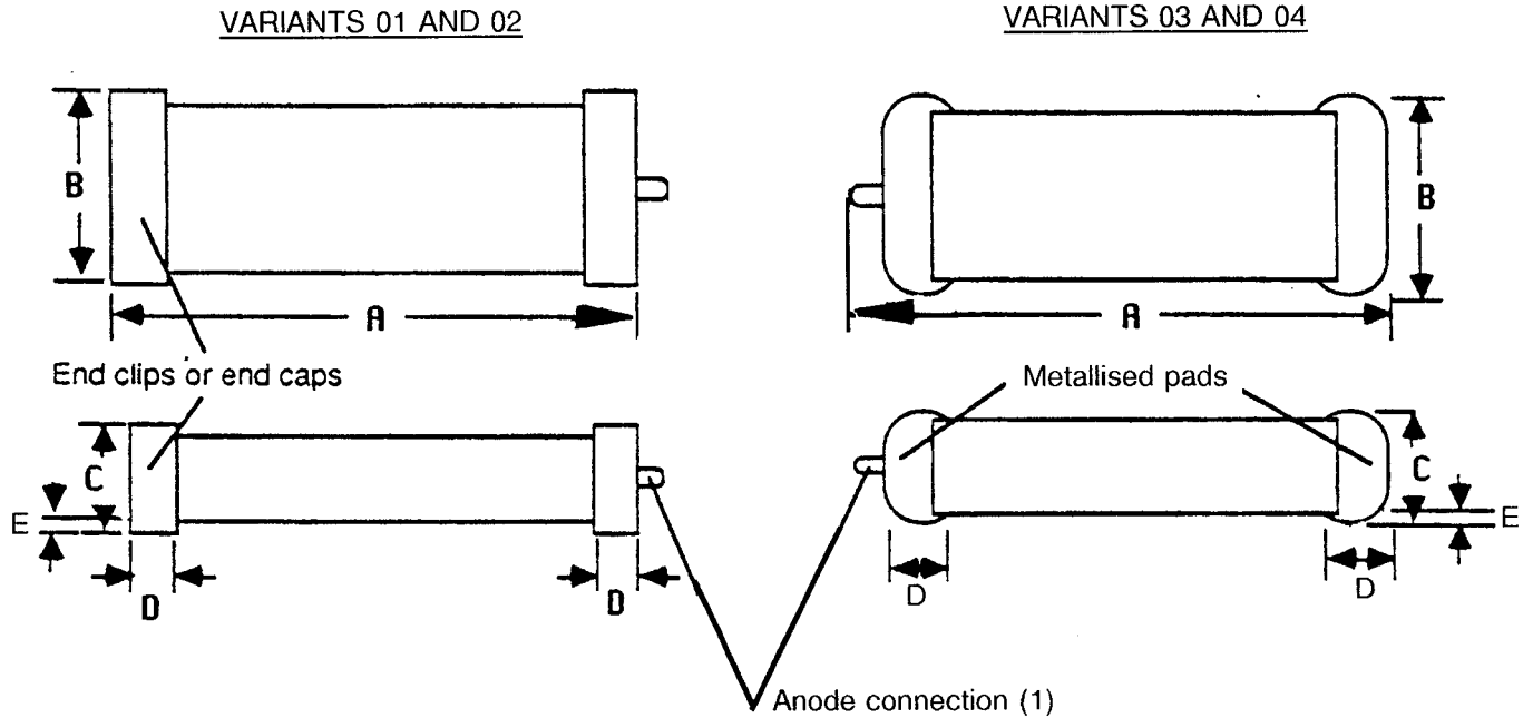
FIGURE 2 - PHYSICAL DIMENSIONS
