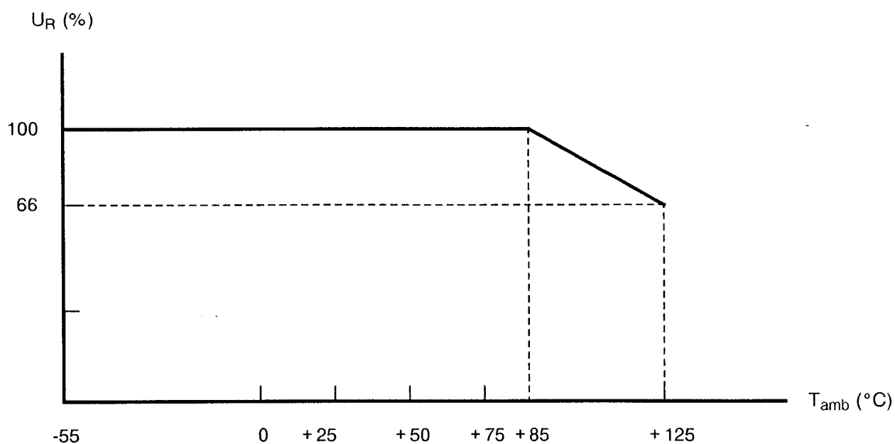
Rated Voltage versus Temperature
