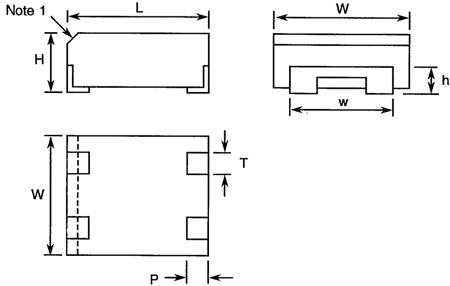
FIGURE 2 - PHYSICAL DIMENSIONS
