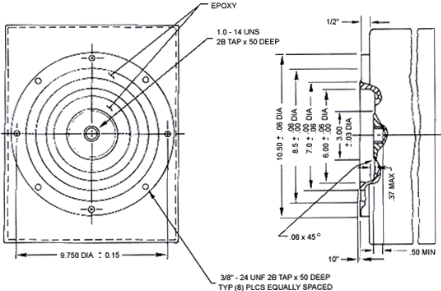
DETAIL E+ FLUSH COVER WITH MODIFIED SCYLLAC
