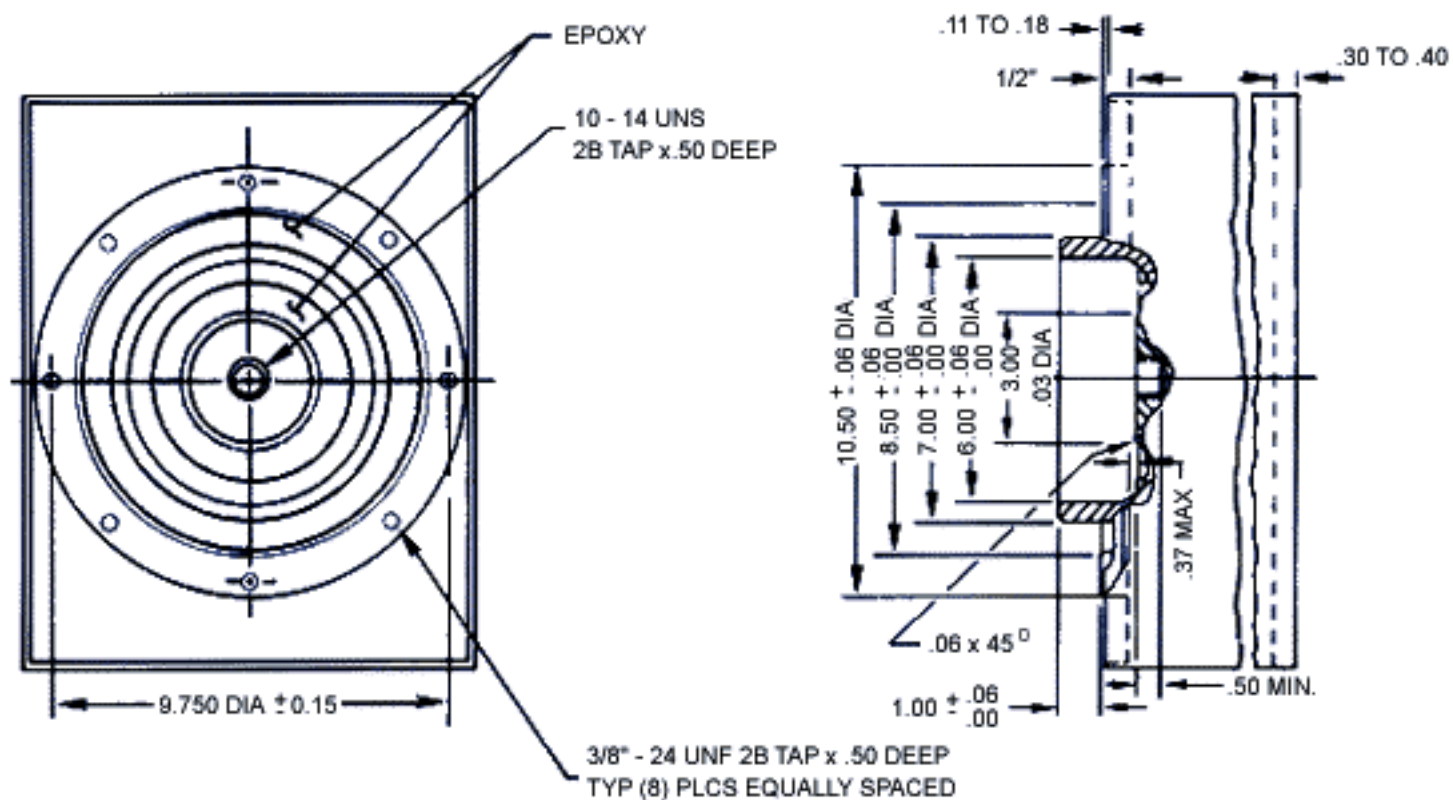
DETAIL F++ RECESSED COVER WITH FULL SCYLLAC
