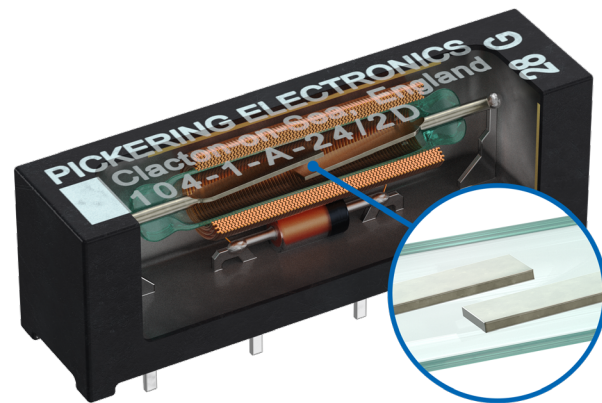
For high-voltage reed relays, the contact is sealed in a vacuum, greatly increasing the minimum standoff and maximum switching voltages. Insulation resistance is high thanks to pin spacing and the relay's base material. As for external shield clearance, this is not an issue when the EM shielding is on the inside of the device.
