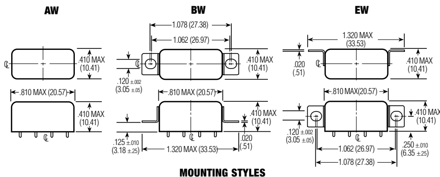
MOUNTING STYLES
