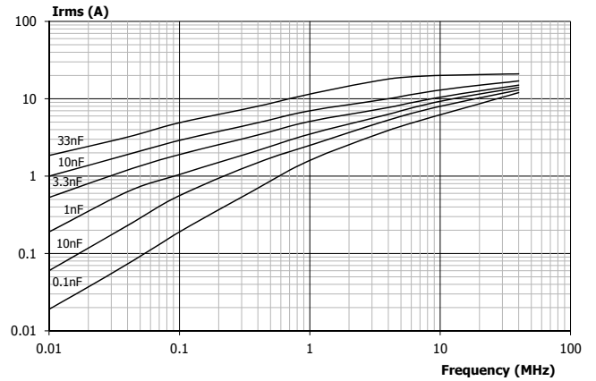
X7R: MAXIMUM ADMISSIBLE CURRENT VS FREQUENCY
