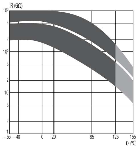
X7R: INSULATION RESISTANCE VS TEMPERATURE
