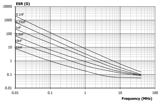
X7R: ESR VS FREQUENCY
