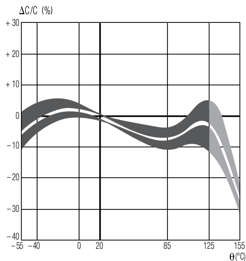
X7R: CAPACITANCE CHANGE VS TEMPERATURE
