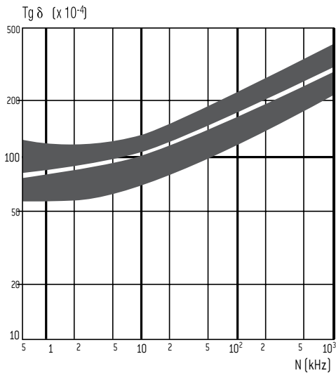
X7R: LOSS TANGENT CHANGE VS FREQUENCY
