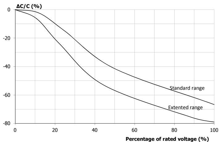
CHANGE VS PERCENTAGE OF RATED VOLTAGE APPLIED
