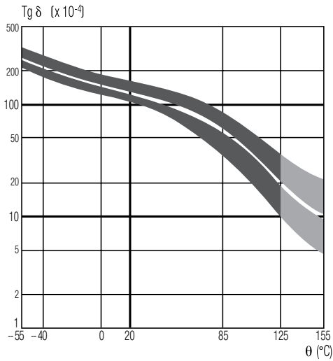
X7R: LOSS TANGENT CHANGE VS TEMPERATURE
