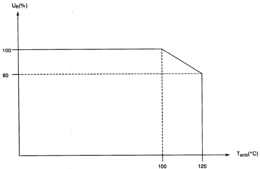
Rated Voltage versus Temperature
