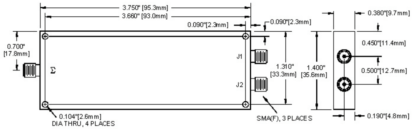
Fig. 12 (Model: PS-C102-2S)
