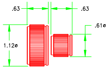
KNOB DETAIL
