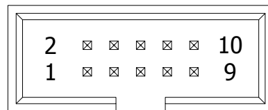
DETAIL A 3M #D2510-6002-AR OR EQUIVALENT
