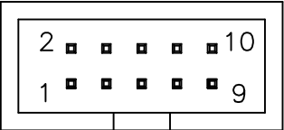
DETAIL A T&B #609-1057
