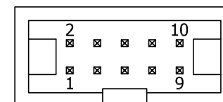
DETAIL A 3M #D2510-6002-AR OR EQUIVALENT
