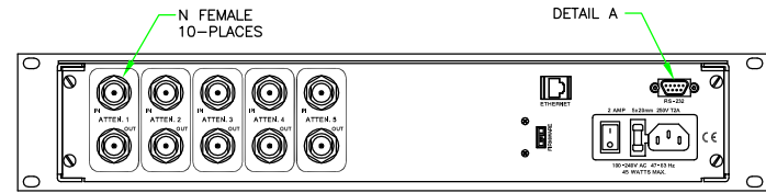
-05 (i.e. 5 ATTENUATORS)
