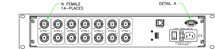
-07 (i.e. 7 ATTENUATORS)
