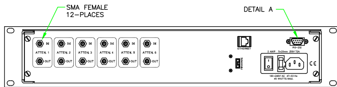
-06 (i.e. 6 ATTENUATORS)
