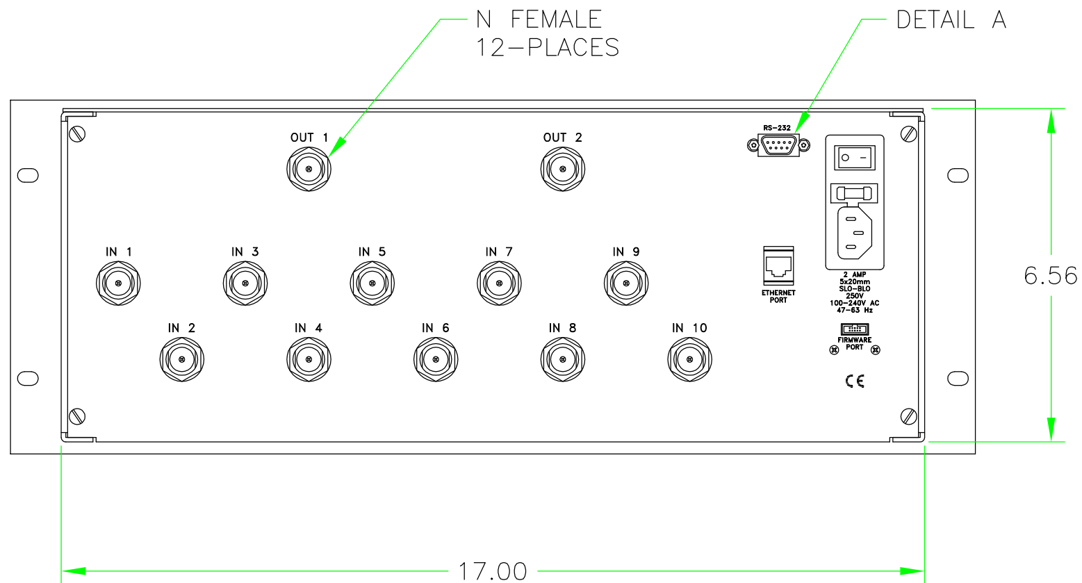
REAR VIEW
