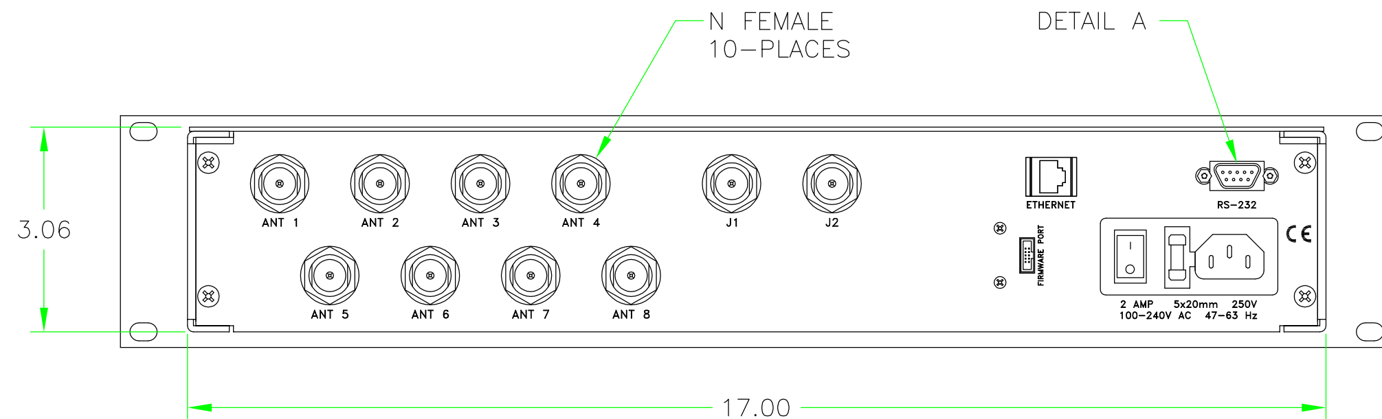
REAR VIEW
