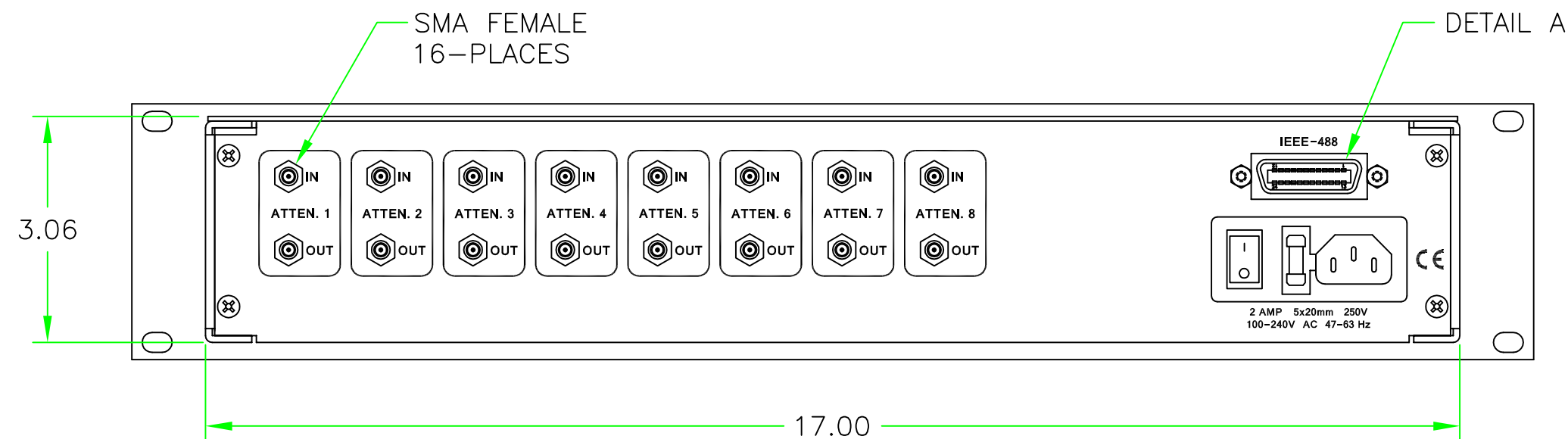
REAR VIEW
