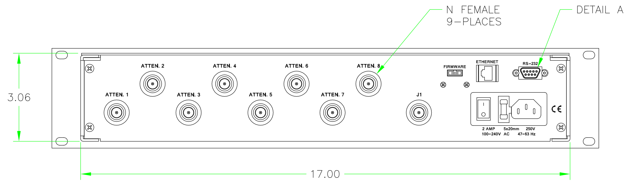
REAR VIEW
