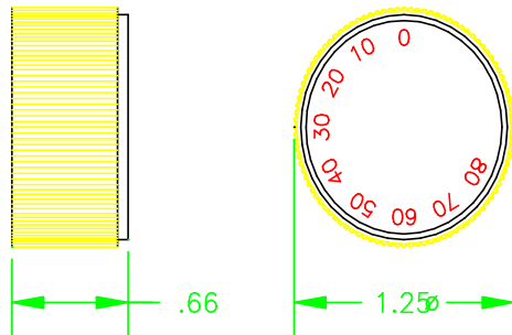
KNOB DETAIL
