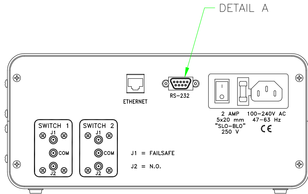
REAR VIEW
