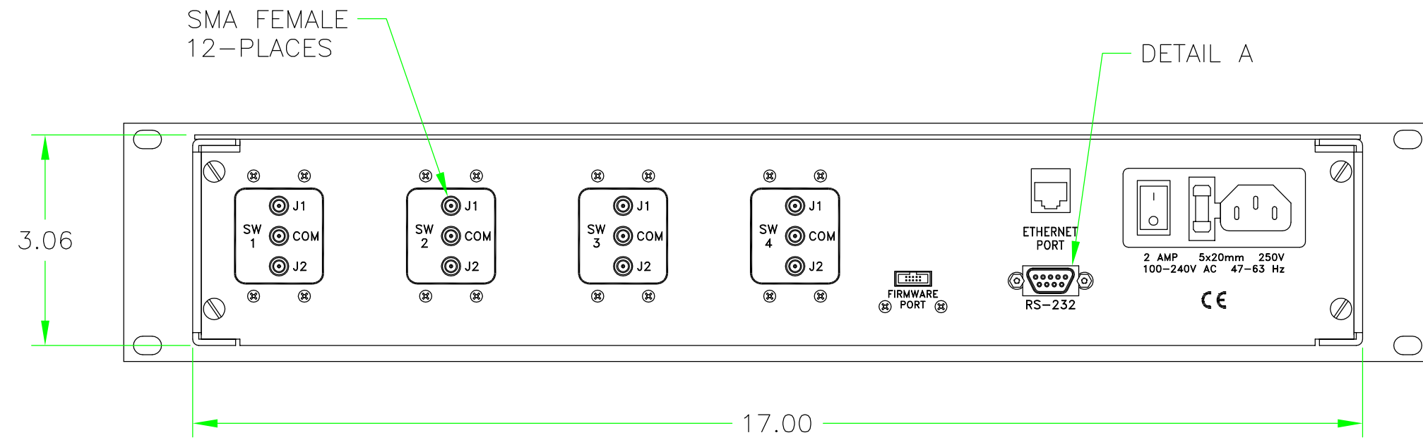
REAR VIEW
