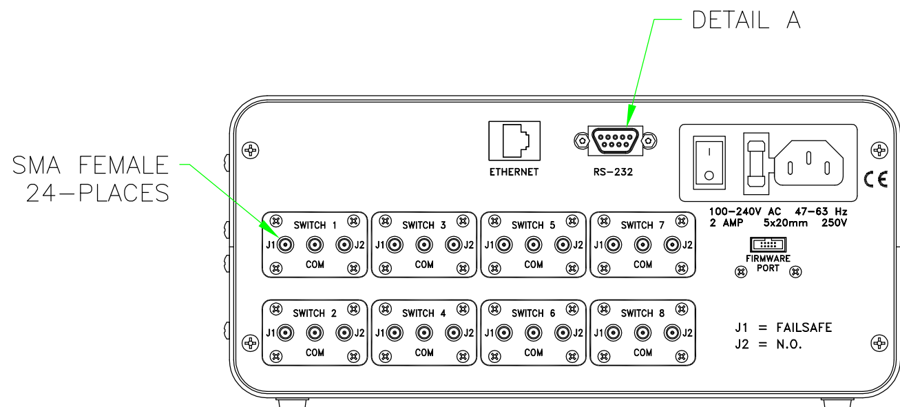
REAR VIEW
