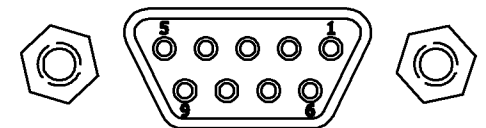
DETAIL A DE-9S
