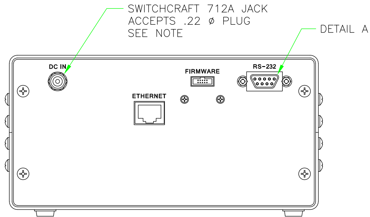
REAR VIEW
