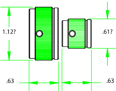
KNOB DETAIL
