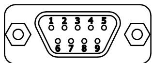
DETAIL A DE-9P
