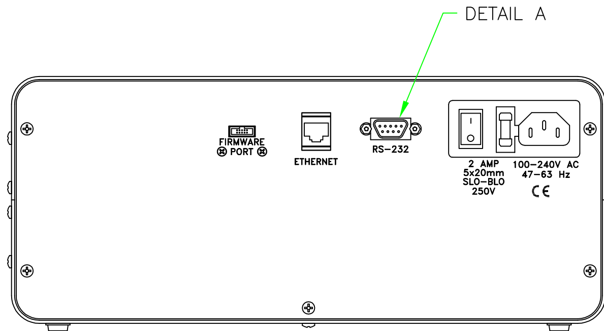
REAR VIEW
