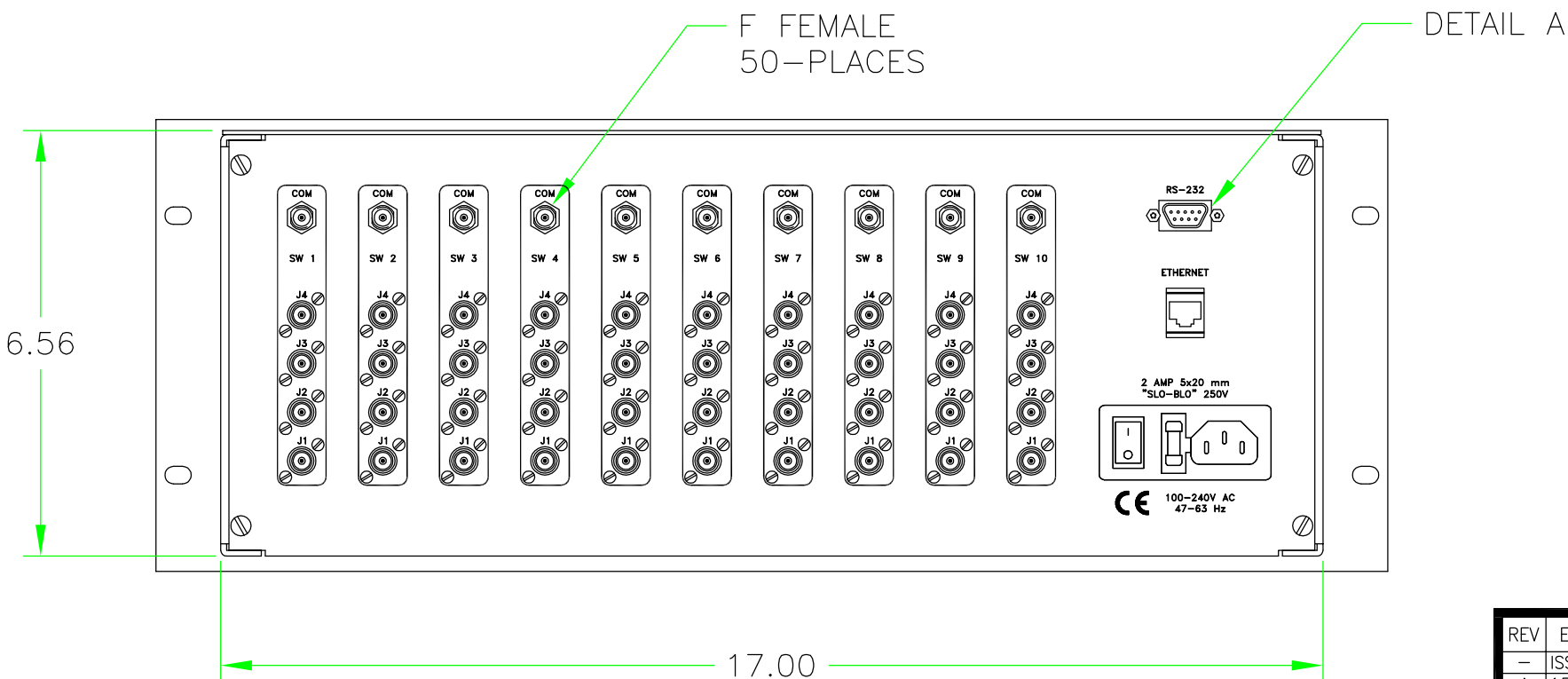
REAR VIEW
