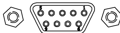
DETAIL A DE-9S
