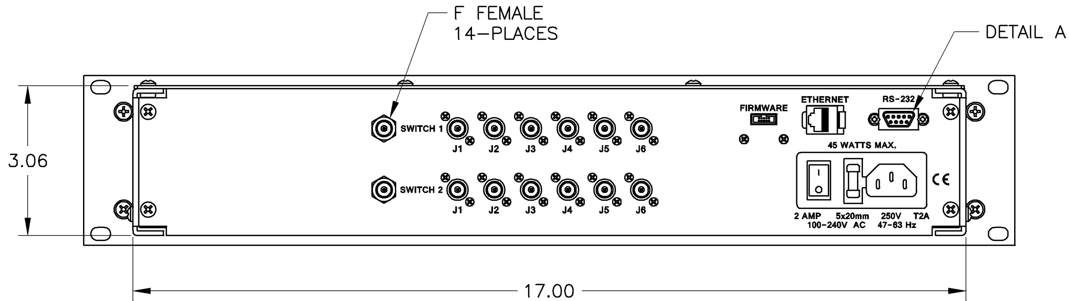
REAR VIEW
