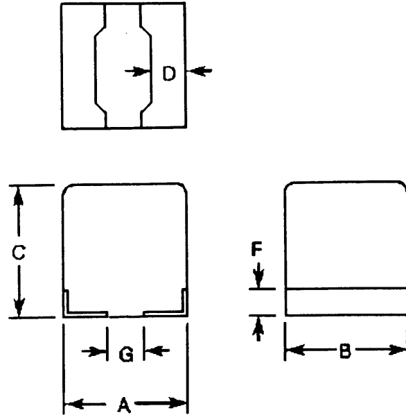
FIGURE 2 - PHYSICAL DIMENSIONS
