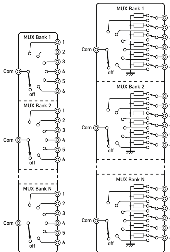
60-800 Unterminated Microwave MUX - up to 16 Multiplexers can be supported
