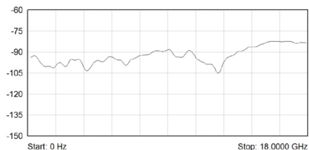
Typical Isolation (dB) Plot for 18 GHz Underterminated Versions
