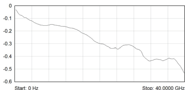
Typical Insertion Loss (dB) Plot for 40 GHz Underterminated Versions
