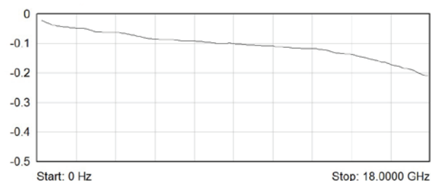
Typical Insertion Loss (dB) Plot for 18 GHz Underterminated Versions
