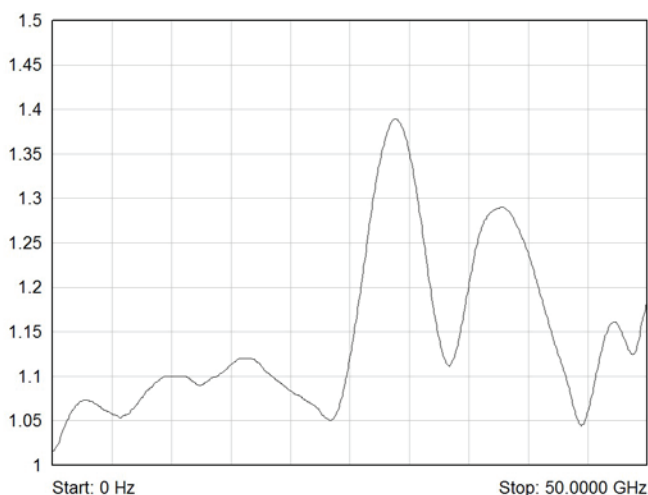
Typical VSWR Plot for 50 GHz Terminated & Underminated Versions
