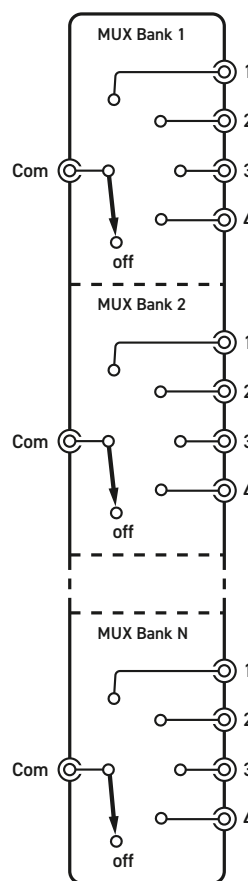
Schematic Diagram for the 60-802 Microwave MUX - up to 16 Multiplexer Modules can be supported
