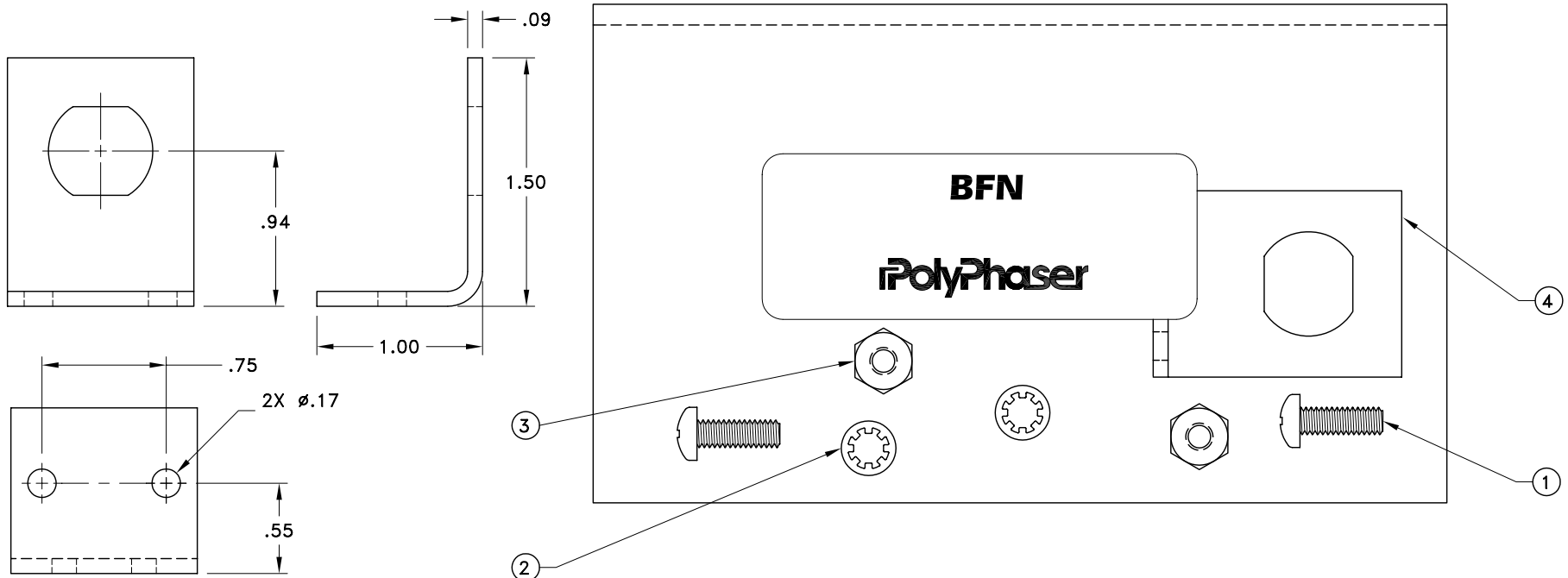
MOUNTING PATTERN
