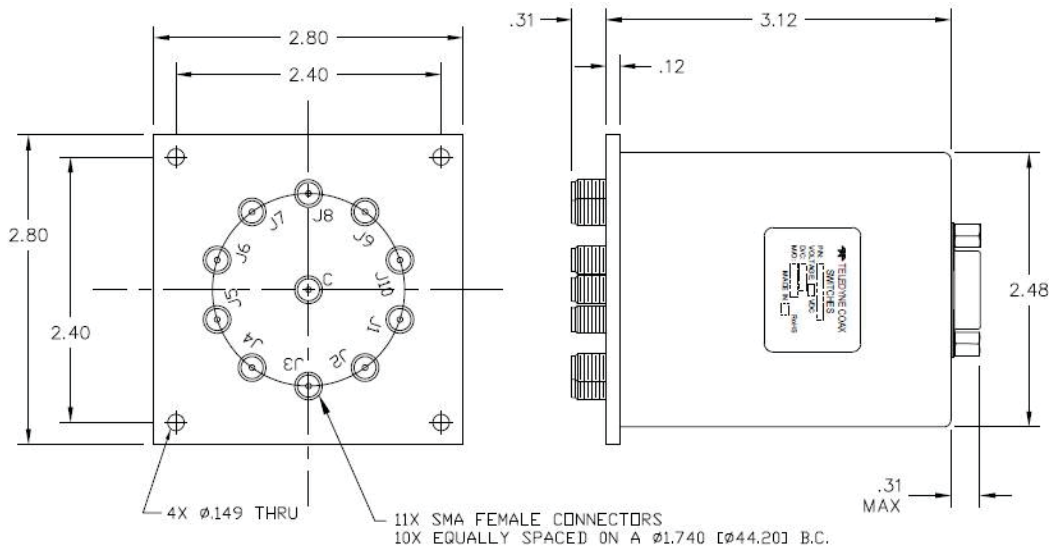
“-TS OR -TDS OPTIONS” 15-PIN D-SUB OR 26-PIN D-MICRO CONNECTOR (EXAMPLE: cCR-58s180-TS OR cCR-58s180-TDS)
