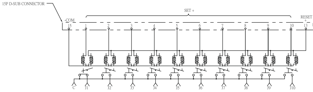
SCHEMATIC COIL 1 SHOWN LAST ENERGIZE
