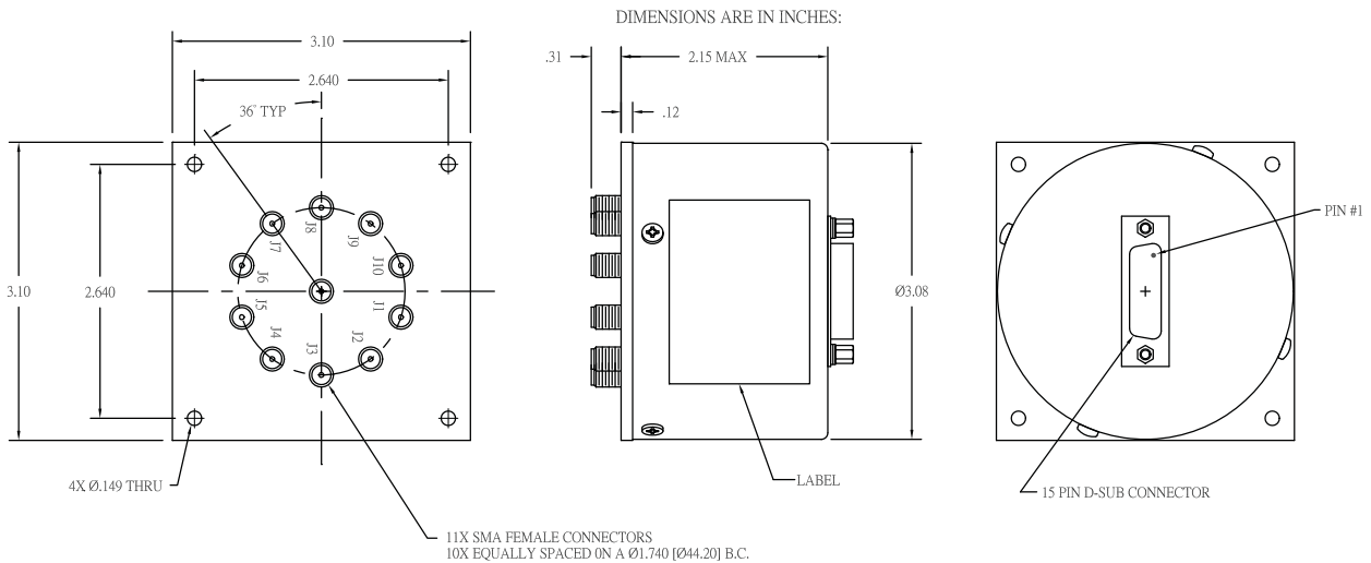
“-S OPTION” 15-PIN D-SUB OR 26-PIN D-MICRO CONNECTOR (EXAMPLE: cCR-58s180-s)
