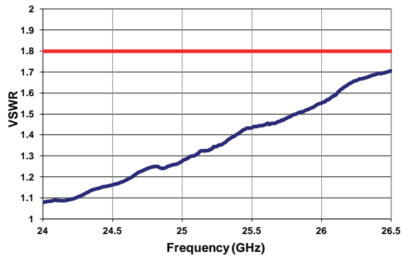
VSWR ( 24-26.5 GHz )
