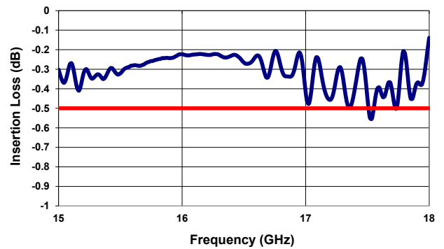
Insertion Loss ( 15-18 GHz )
