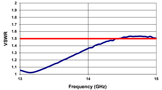
VSWR ( 13-15 GHz )
