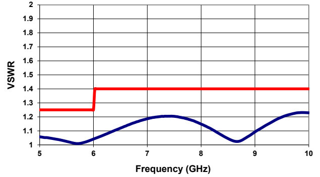
VSWR ( 5-10 GHz )
