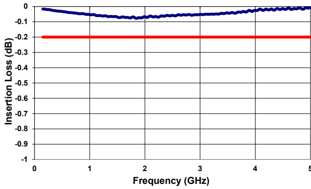
Insertion Loss ( DC-5 GHz )
