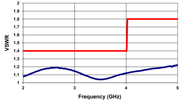
VSWR ( 2-5 GHz )
