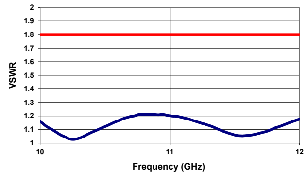
VSWR ( 10-12 GHz )
