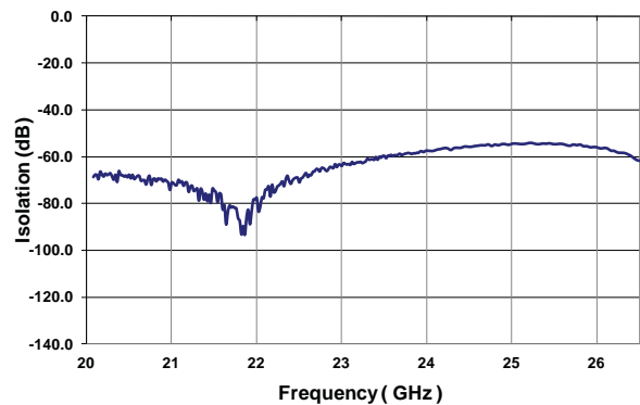
Isolation (20-26.5 GHz)
