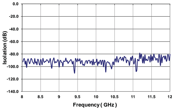
Isolation (8-12 GHz)
