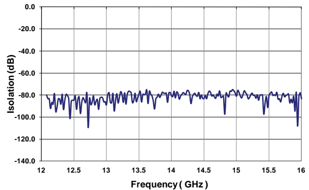
Isolation (12-16 GHz)
