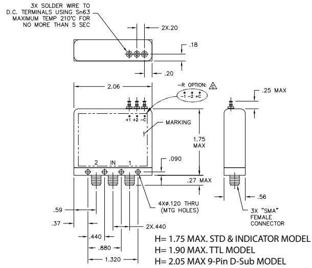
POWER INPUT TERMINALS
