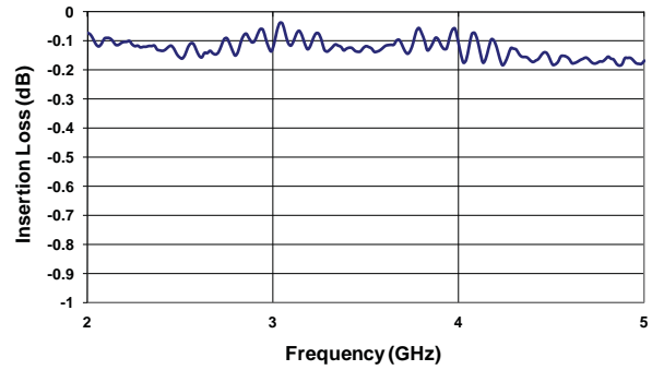
Insertion Loss (2-5 GHz)
