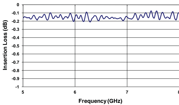
Insertion Loss (5-8 GHz)
