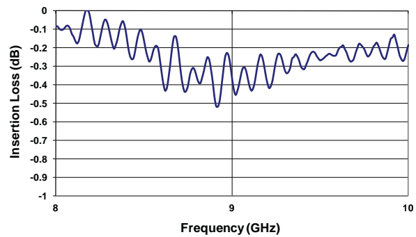
Insertion Loss (8-10 GHz)
