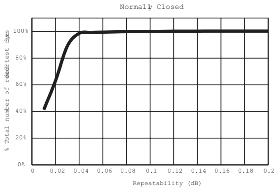
REPEAT ABILITY CHARACTERISTICS SGRF303 RELAYS
