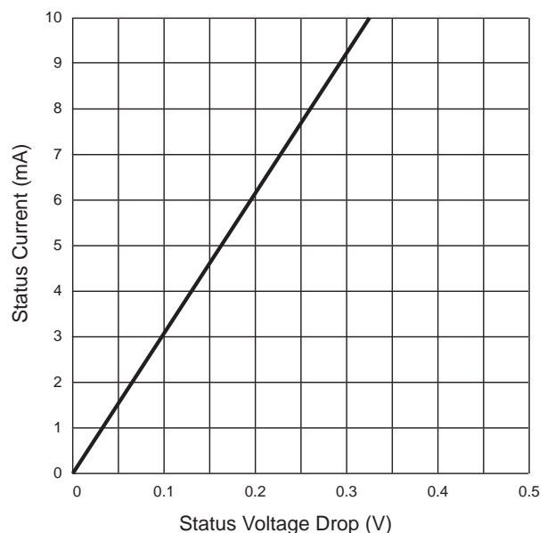
Figure 3 — 2305115-2T status current vs. voltage
