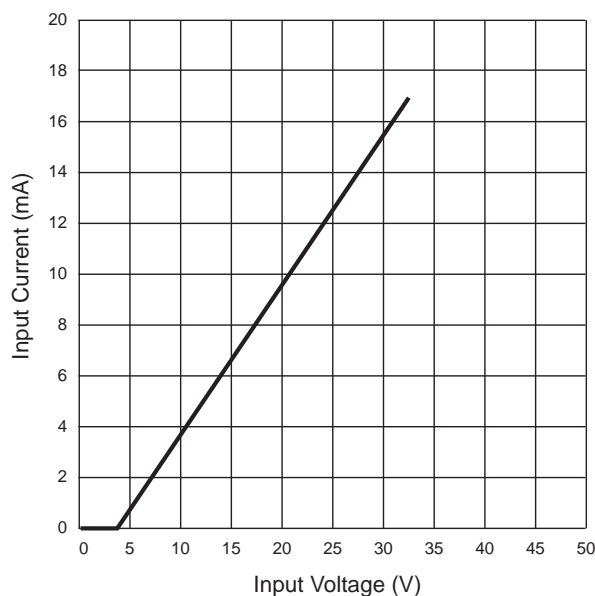
Figure 2 — 2305115-2T input current vs. voltage
