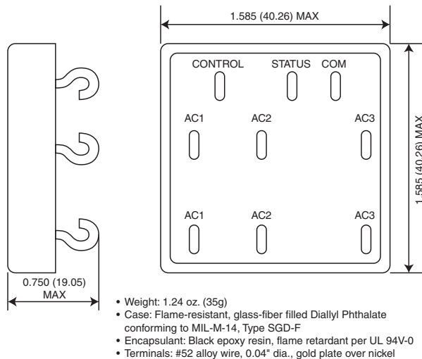
Figure 1 – 2305115-2T mechanical specification; dimensions in inches (mm)
