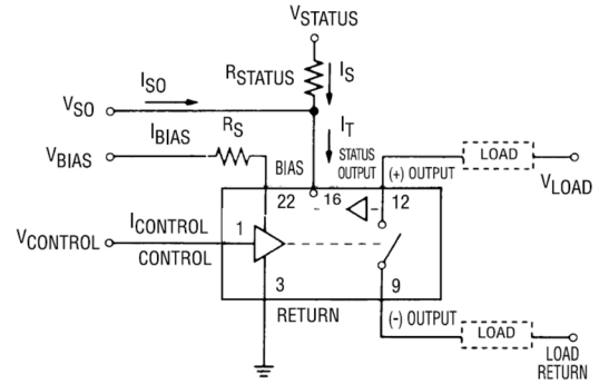
3 TERMINAL INPUT WITH STATUS (See Note 5)
