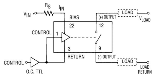
2 TERMINAL INPUT (OPEN COLLECTOR TTL DRIVE)
