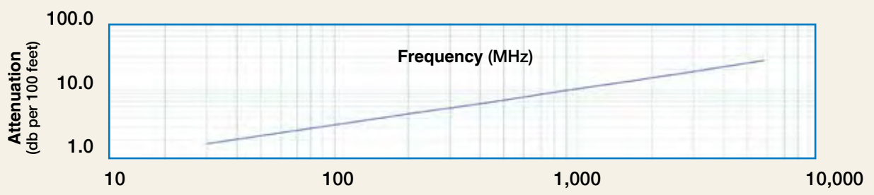
Attenuation vs. Frequency (typical)
